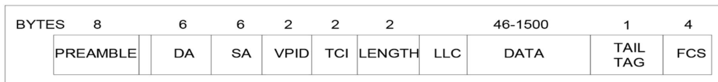
Figure 12. Tail Tag Frame Format
